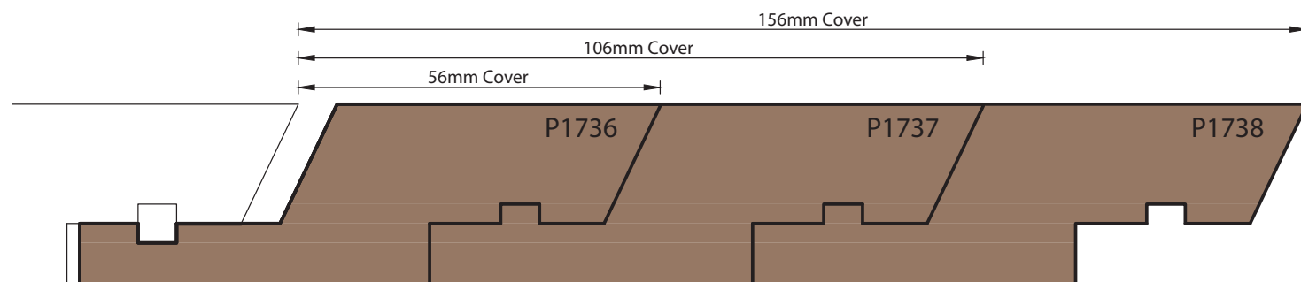
Random Width & Depth (Combination Rusticated Profile)
