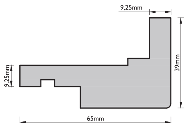
P330 External Corner Moulding
