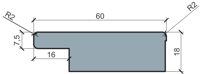
PI340 - 60X18mm
