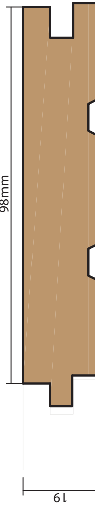
P3396 98X19mm Flooring
