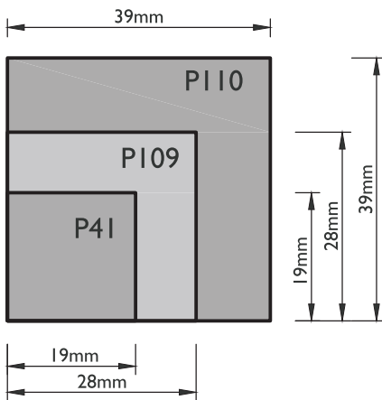
Eaves Moulding
