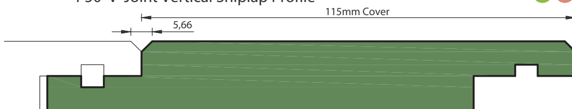
P50 'V' Joint Vertical Shiplap Profile
