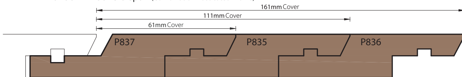
Random Width & Depth (Combination Rusticated Profile)
