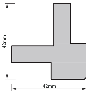
P32I External Corner Moulding
