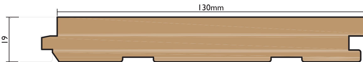
P8816 130X19mm Flooring
