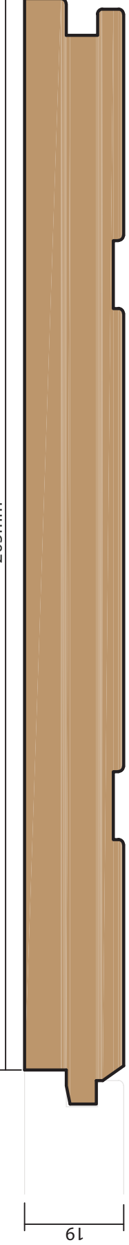
P8821 205X19mm Flooring
