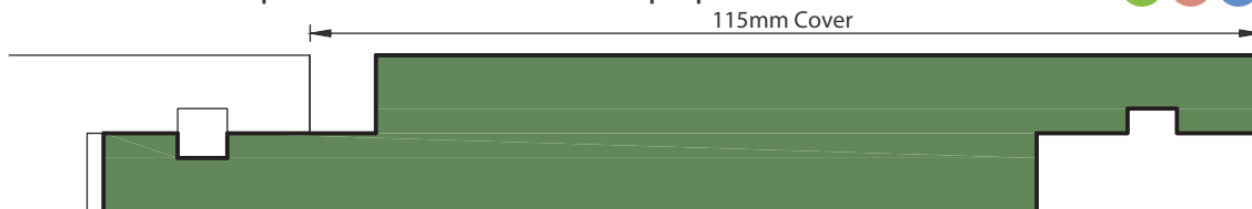
P55 Square Grooved Vertical Shiplap Profile
