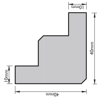
P40 External Corner Moulding
