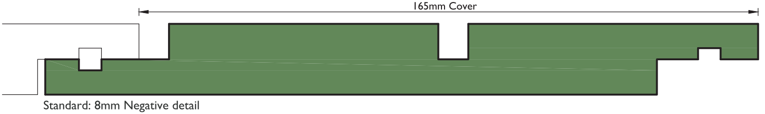
P59 Square Grooved Vertical Shiplap Profiles
