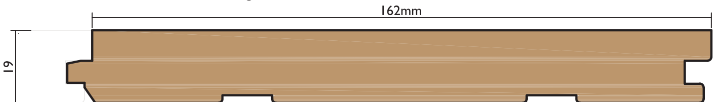
P8817 162X19mm Flooring
