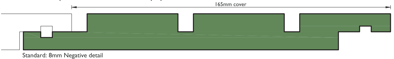
P60 Square Grooved Vertical Shiplap Profiles
