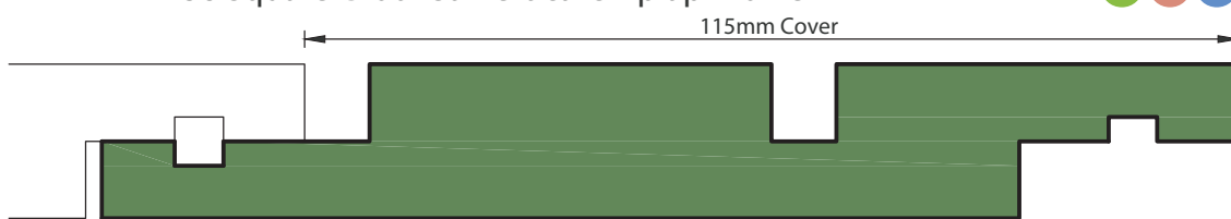
P58 Square Grooved Vertical Shiplap Profile
