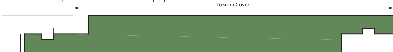
P56 Square Grooved Vertical Shiplap Profile
