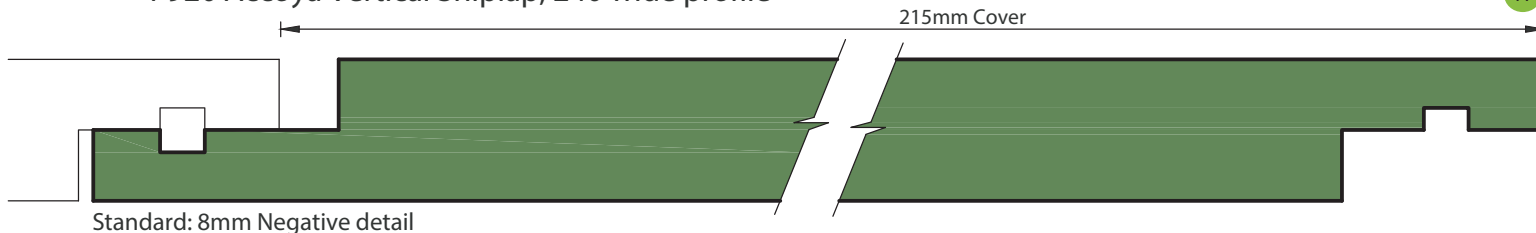
P920 Accoya Vertical Shiplap, 240 wide profile
