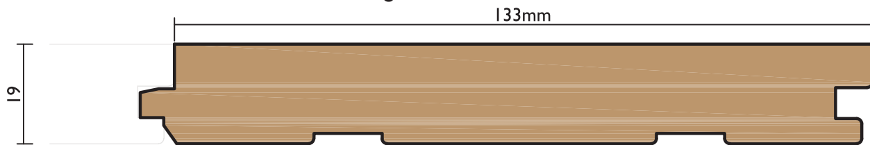
P8812 133X19mm Flooring
