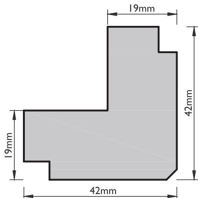
P32I External Corner Moulding
