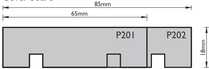
Cover board
