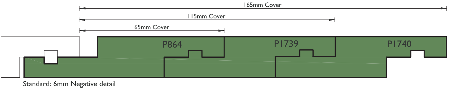
Random Series (Combination Profiles 6mm negative detail)
