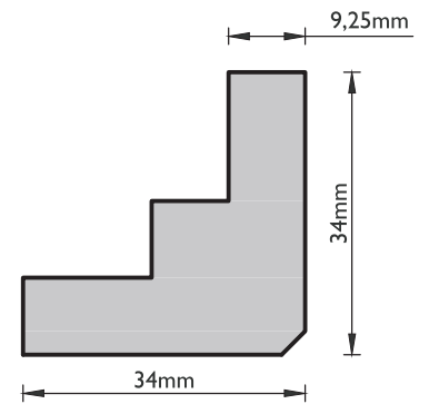
P330 External Corner Moulding
