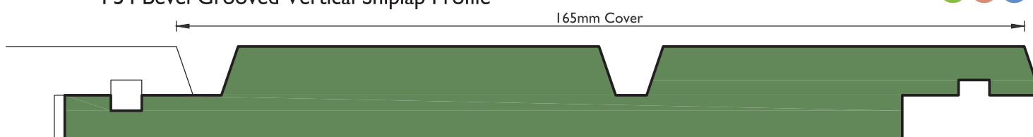
P54 Bevel Grooved Vertical Shiplap Profile
