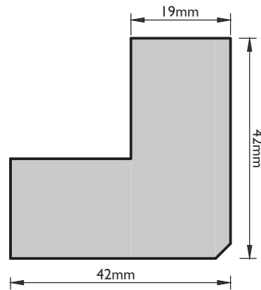
P42 External Corner Moulding
