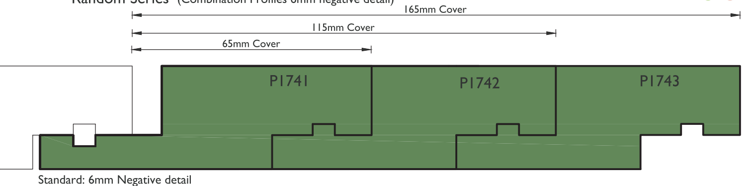
Random Series (Combination Profiles 6mm negative detail)
